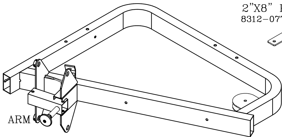
F-1 [1PCS] LEFT PEC ARM
